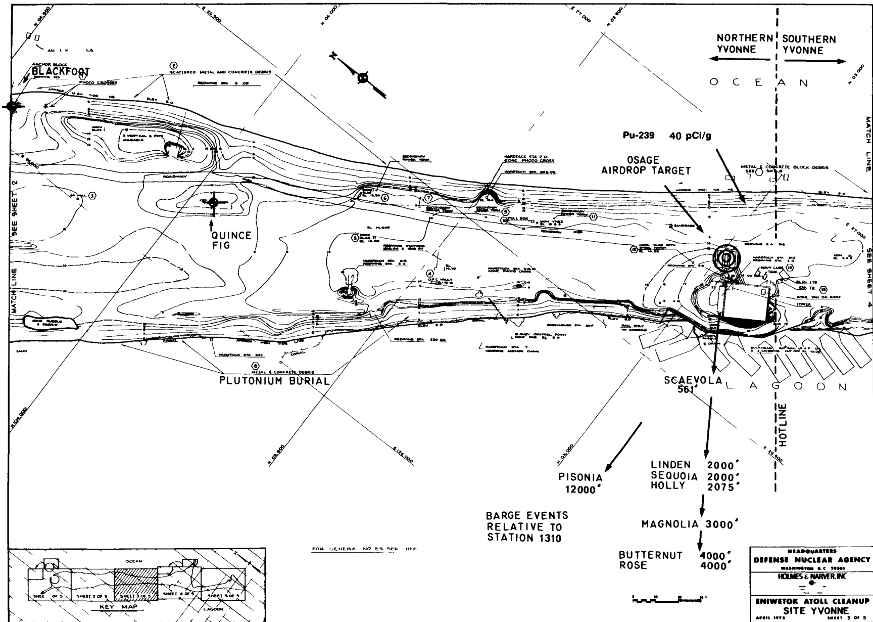
FIGURE 65 SITE YVONNE, SHEET 3 OF 5, SOUTH END
